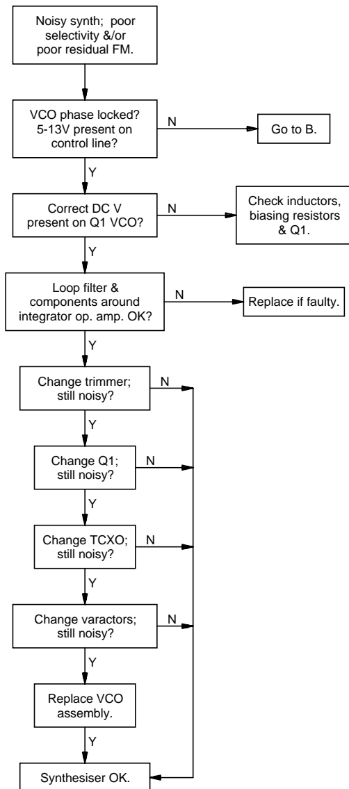
D (Refer to synth. & VCO circuit diagrams)
